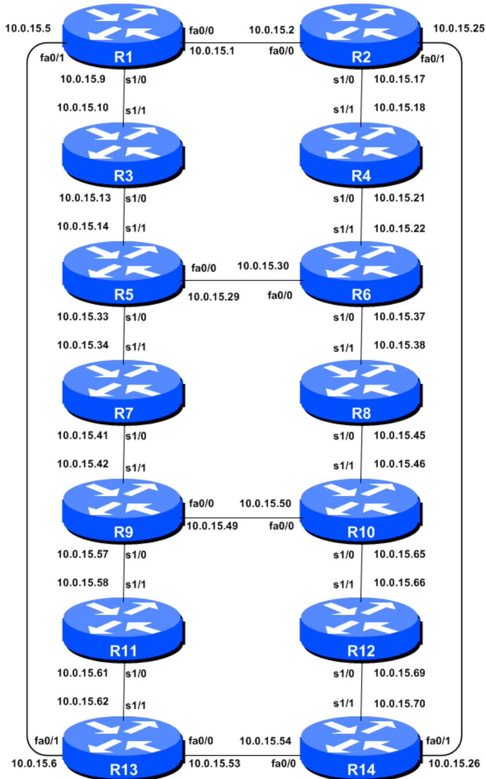
Figure 1 – Addressing Scheme for Modules 1 to 5
